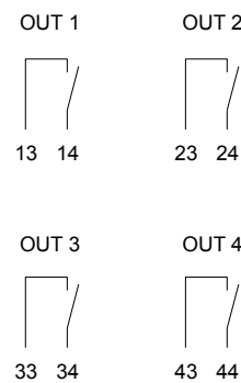
Connessione uscite statiche Solid state relay outputs connection
